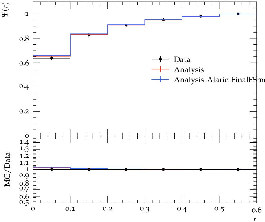
Jet shape \Psi for p_{\perp} \in 110\text{--}160\text{ GeV} , y \in 1.2\text{--}2.1
