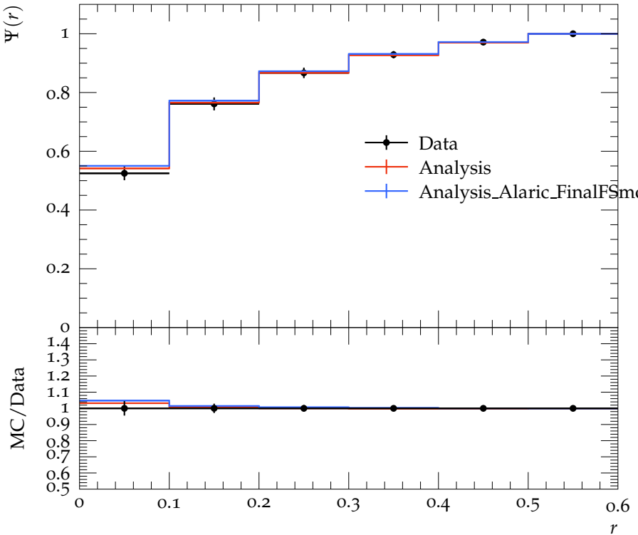
Jet shape \Psi for p_{\perp} \in 60\text{--}80\text{ GeV} , y \in 1.2\text{--}2.1
