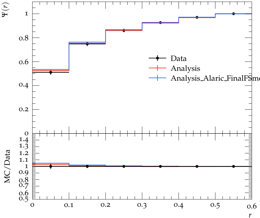
Jet shape \Psi for p_{\perp} \in 60\text{--}80\text{ GeV} , y \in 0.0\text{--}0.3
