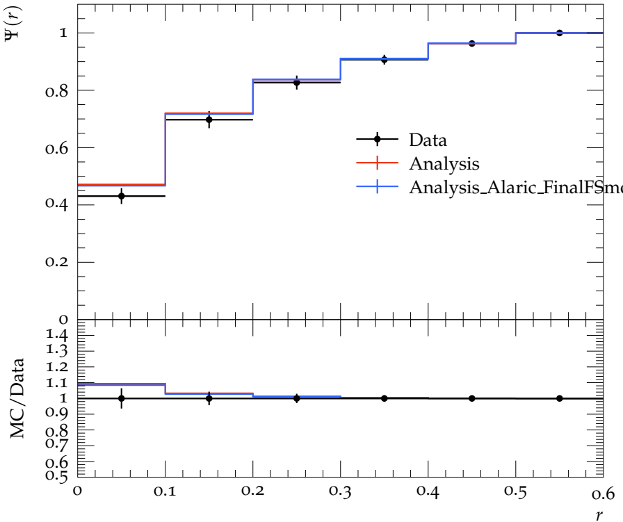
Jet shape \Psi for p_{\perp} \in 40\text{--}60\text{ GeV} , y \in 1.2\text{--}2.1
