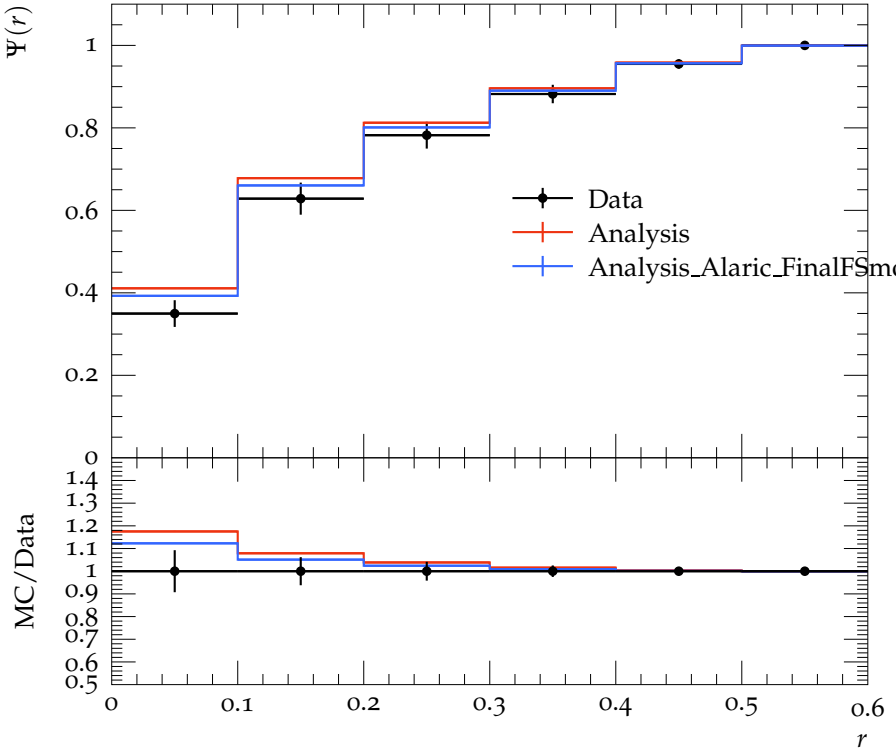
Jet shape \Psi for p_{\perp} \in 30\text{--}40\text{ GeV} , y \in 1.2\text{--}2.1
