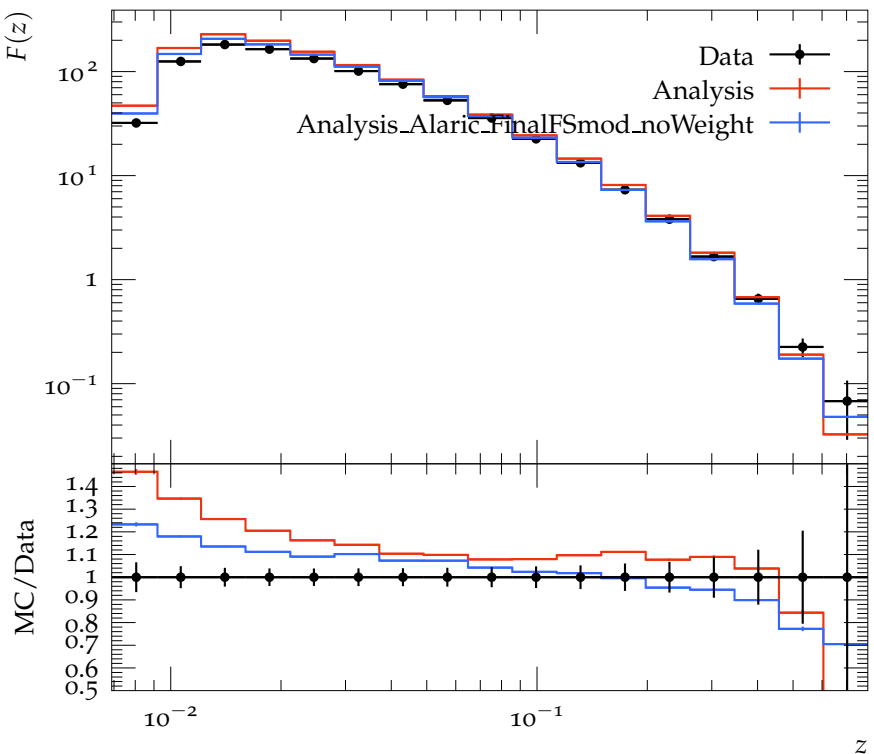
F(z) for 40 \text{ GeV} < p_{T \text{ jet}} < 60 \text{ GeV}
