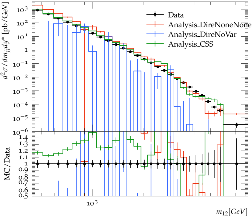
Dijet cross section ( 1.0 \leq y^* < 1.5 ), R=0.4
