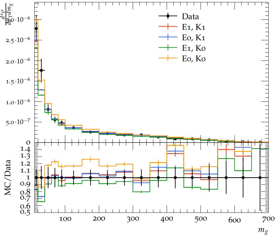
CMS, 13 TeV, Groomed jet mass m_g ( p_T > 1300 GeV)
