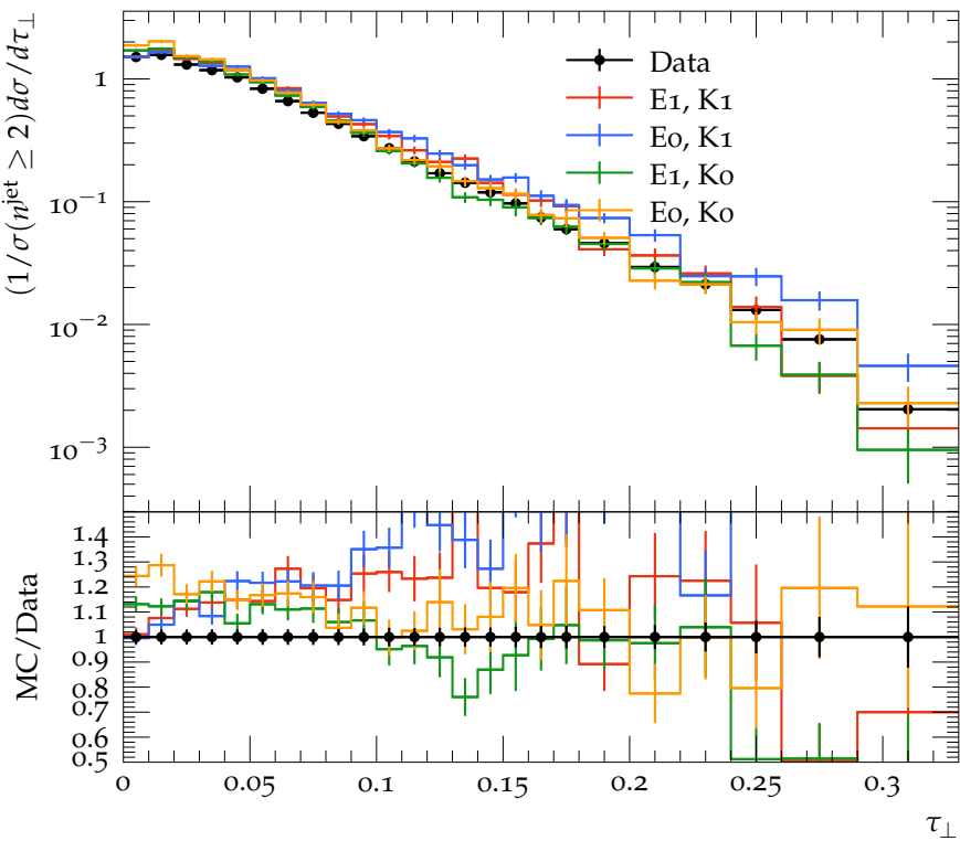
Transverse Thrust for n^{\text{jet}} = 4, H_{T2} > 2.0 \text{ TeV}
