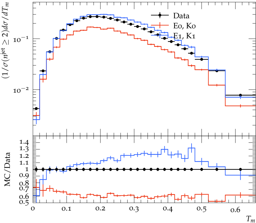
Thrust Minor for n^{\text{jet}} = 4 , 1.0 \text{ TeV} < H_{T2} < 1.5 \text{ TeV}
