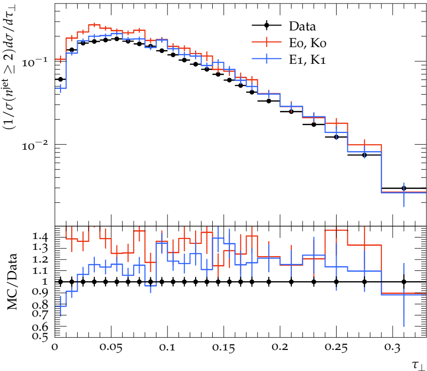
Transverse Thrust for n^{\text{jet}} = 5 , 1.5 \text{ TeV} < H_{T2} < 2.0 \text{ TeV}
