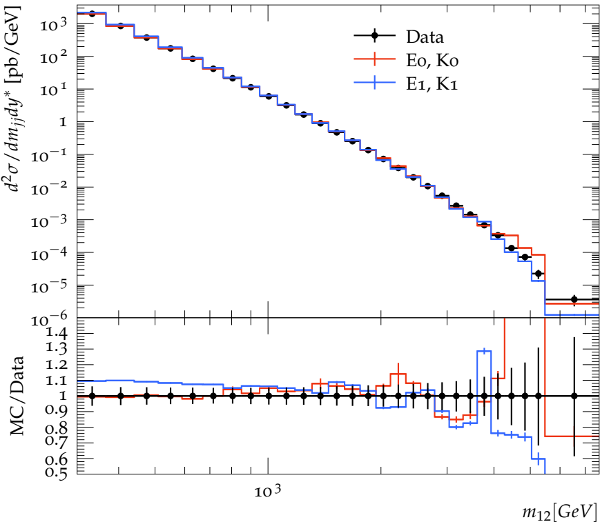
Dijet cross section ( 0.5 \leq y^* < 1.0 ), R=0.4
