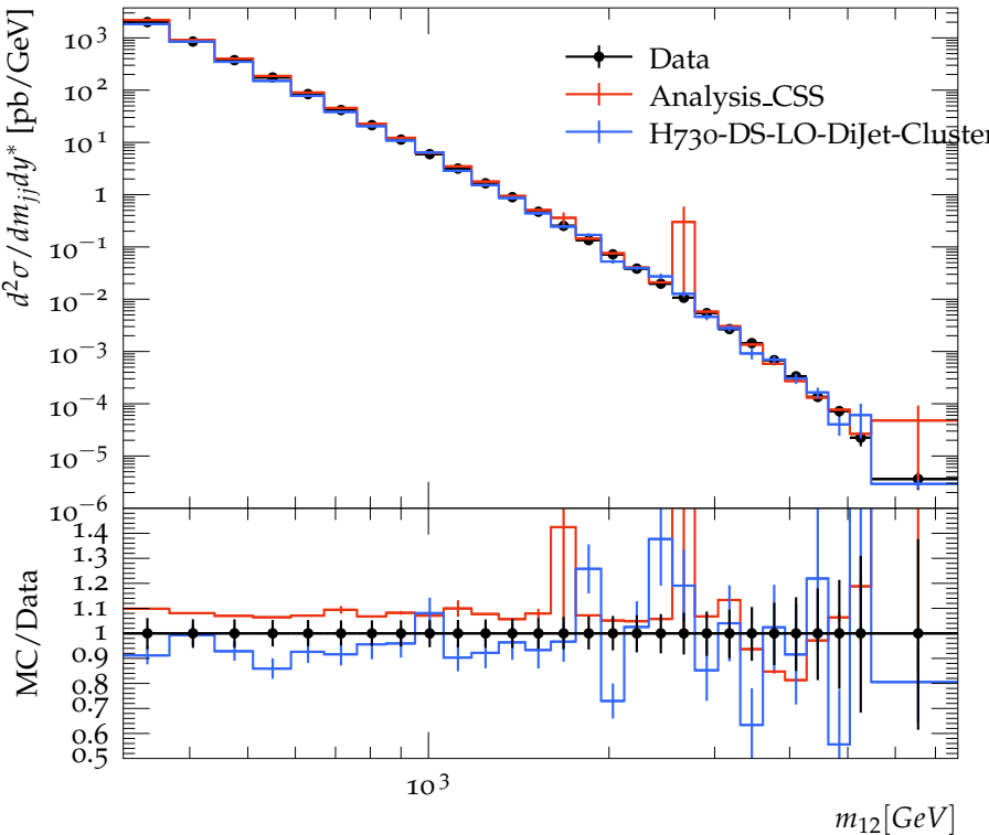
Dijet cross section ( 0.5 \leq y^* < 1.0 ), R=0.4
