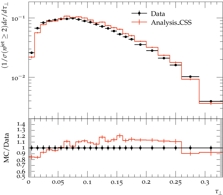
Transverse Thrust for n^{\text{jet}} = 5, 1.0 \text{ TeV} < H_{T2} < 1.5 \text{ TeV}
