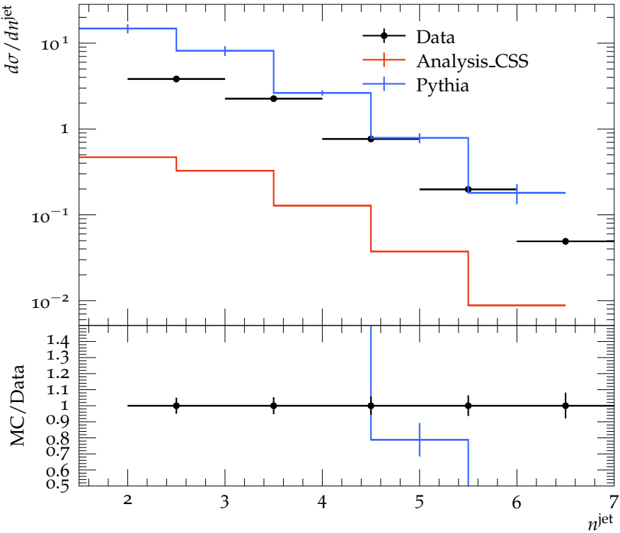
Jet multiplicity for H_{T2} > 2.0 TeV
