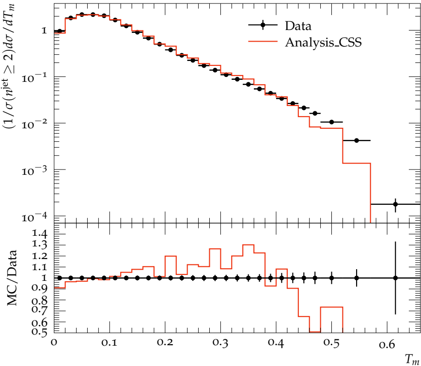
Thrust Minor for n^{\text{jet}} = 3, H_{T2} > 2.0 TeV
