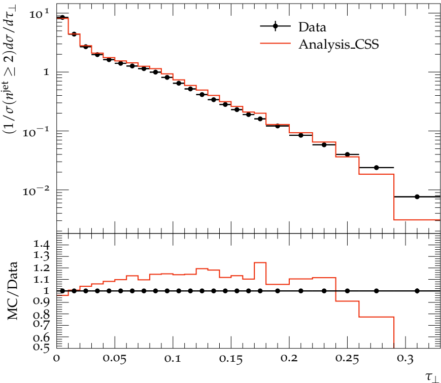
Transverse Thrust for n^{\text{jet}} = 3, 1.0 \text{ TeV} < H_{T2} < 1.5 \text{ TeV}
