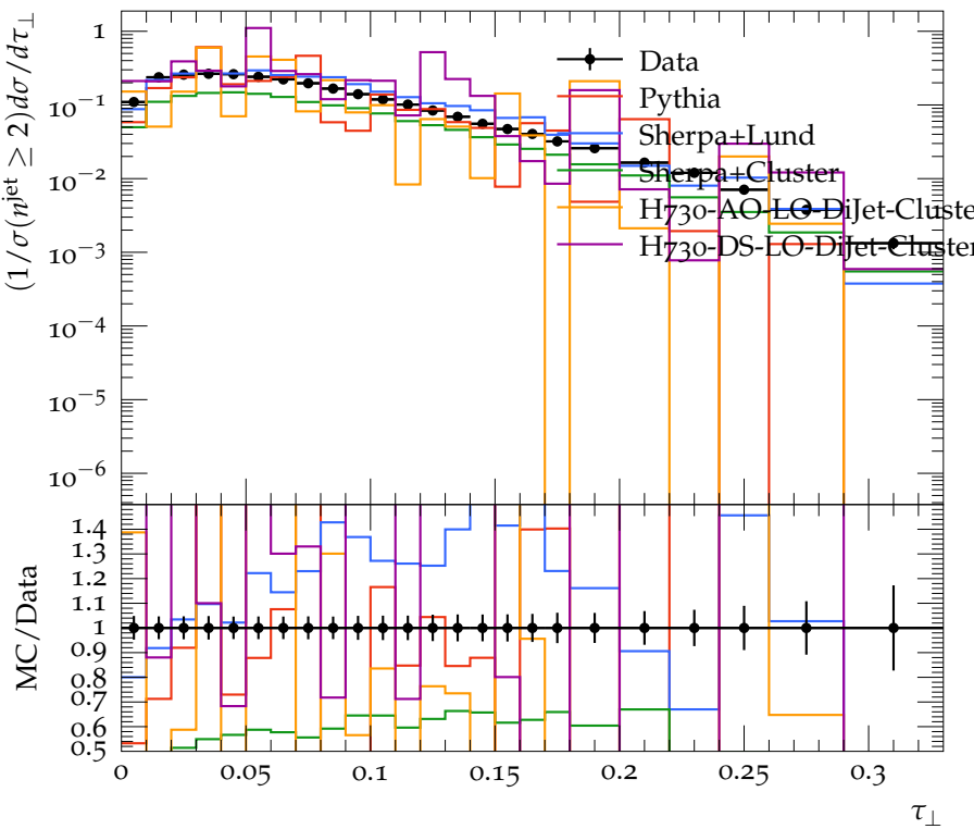
Transverse Thrust for n^{\text{jet}} = 5, H_{T2} > 2.0 \text{ TeV}
