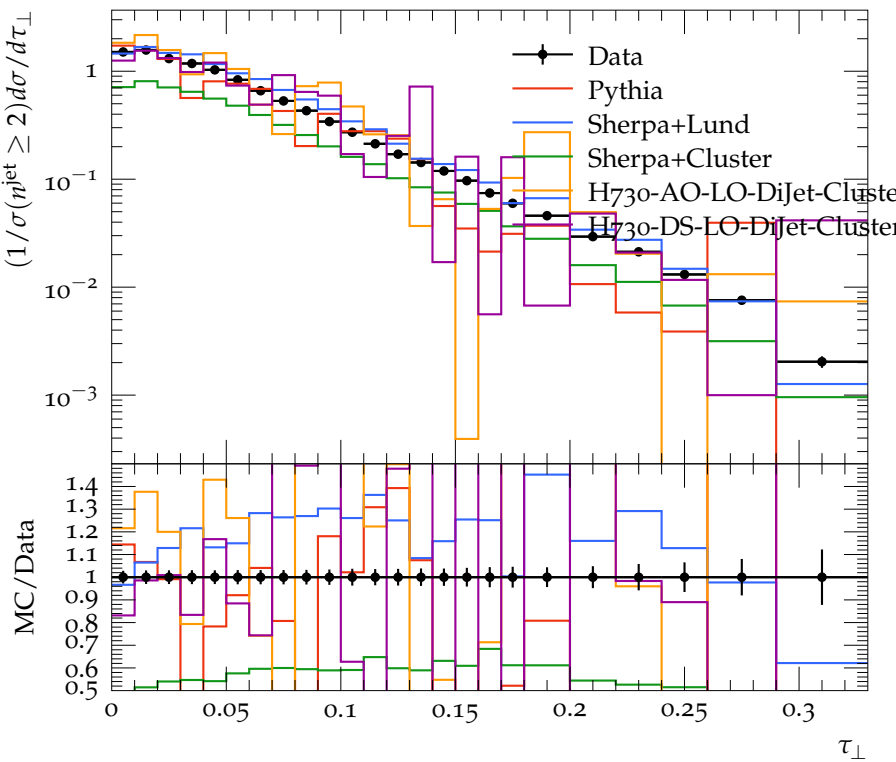
Transverse Thrust for n^{\text{jet}} = 4 , H_{T2} > 2.0 TeV
