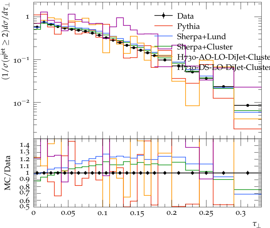
Transverse Thrust for n^{\text{jet}} = 4 , 1.0 \text{ TeV} < H_{T2} < 1.5 \text{ TeV}
