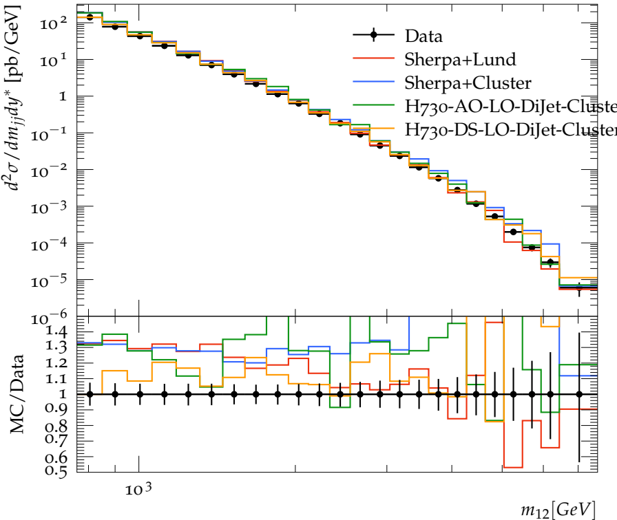
Dijet cross section ( 1.5 \leq y^* < 2.0 ), R=0.4
