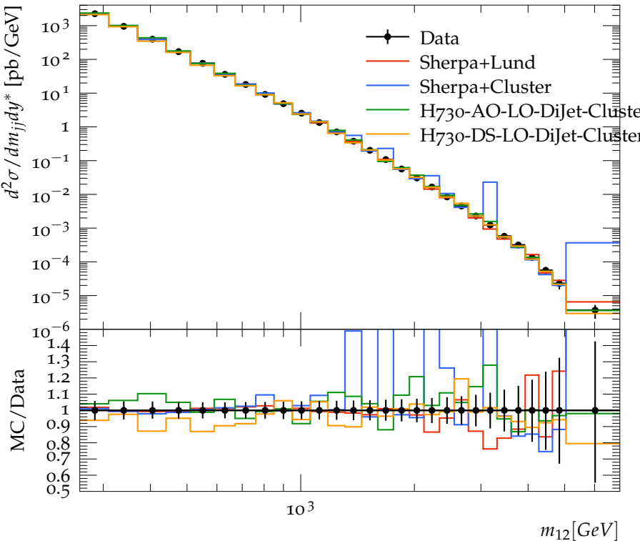
Dijet cross section ( y^* < 0.5 ), R=0.4
